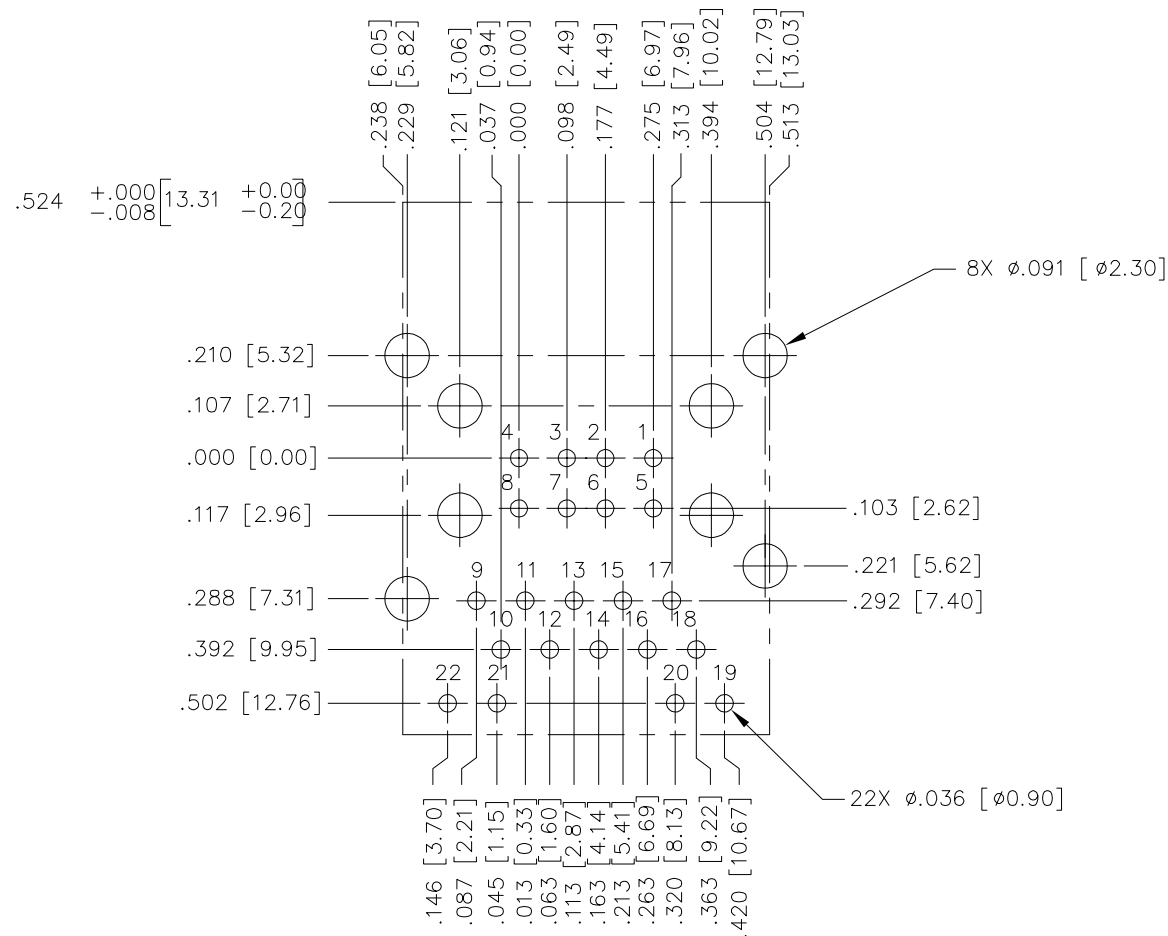
SUGGESTED FOOTPRINT (SHOWN FROM COMPONENT SIDE)
